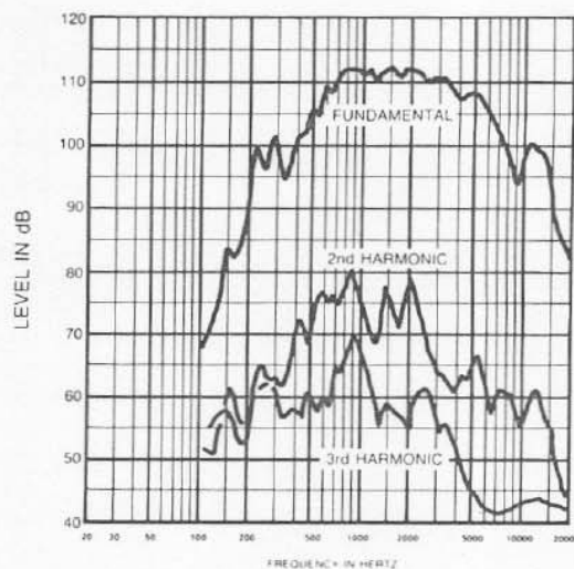
FIGURE 3 848AT Frequency Response (1 watt at 1 meter)
