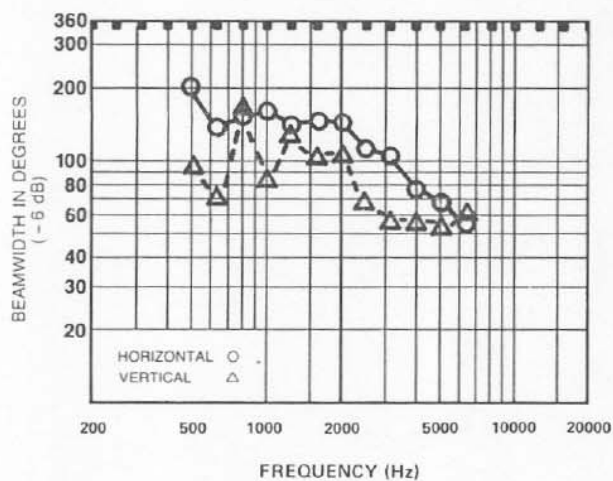
FIGURE 2 848AT Beamwidth vs. Frequency
